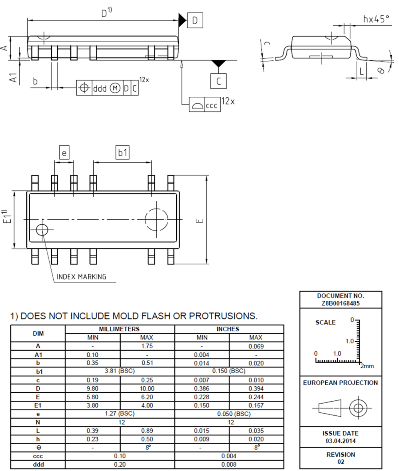
Figure 39 PG-DSO-12
