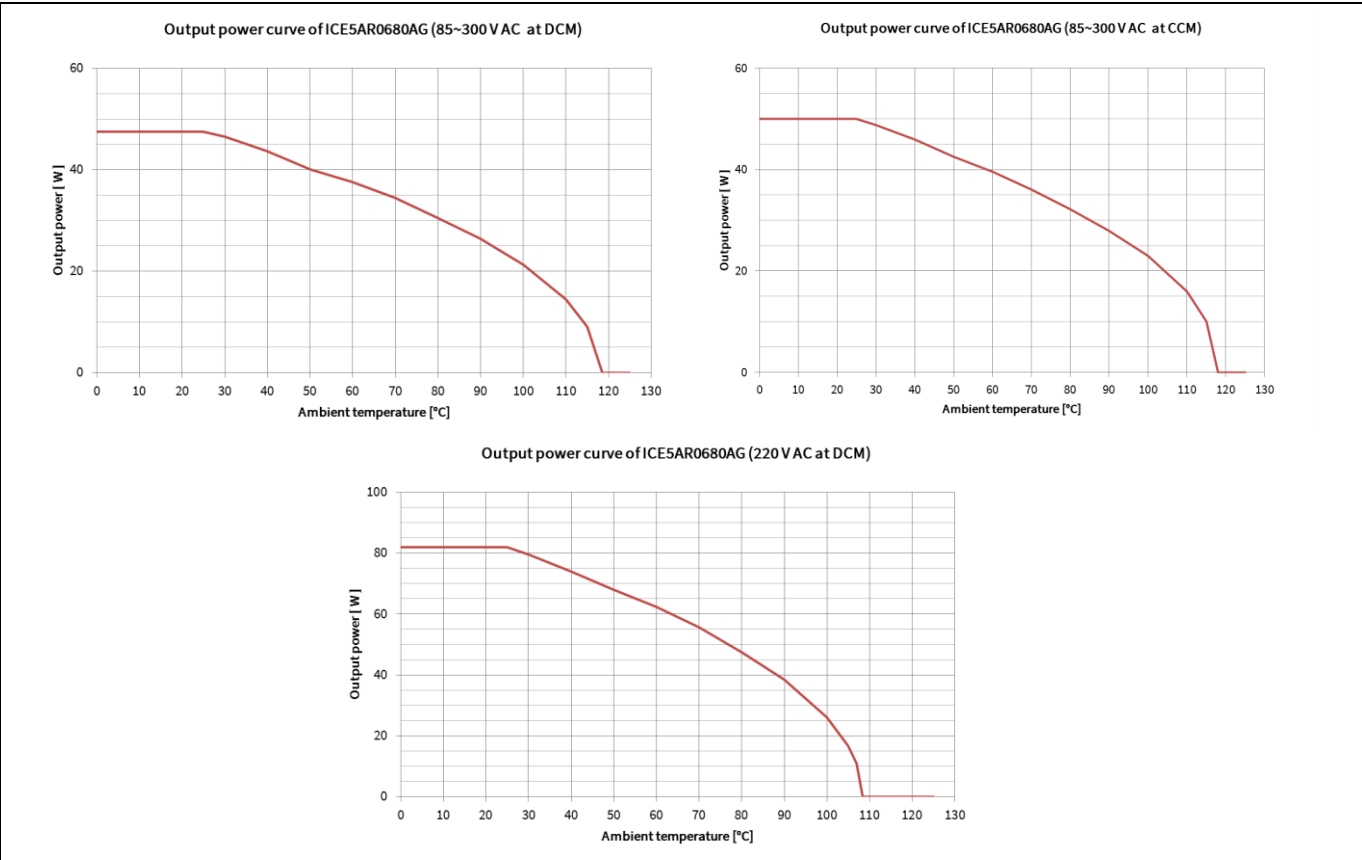
Figure 38 Output power curve of ICE5AR0680AG
