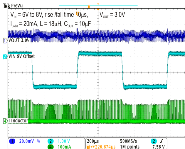
LINE TRANSIENT RESPONSE FOR 3V OUTPUT VOLTAGE
