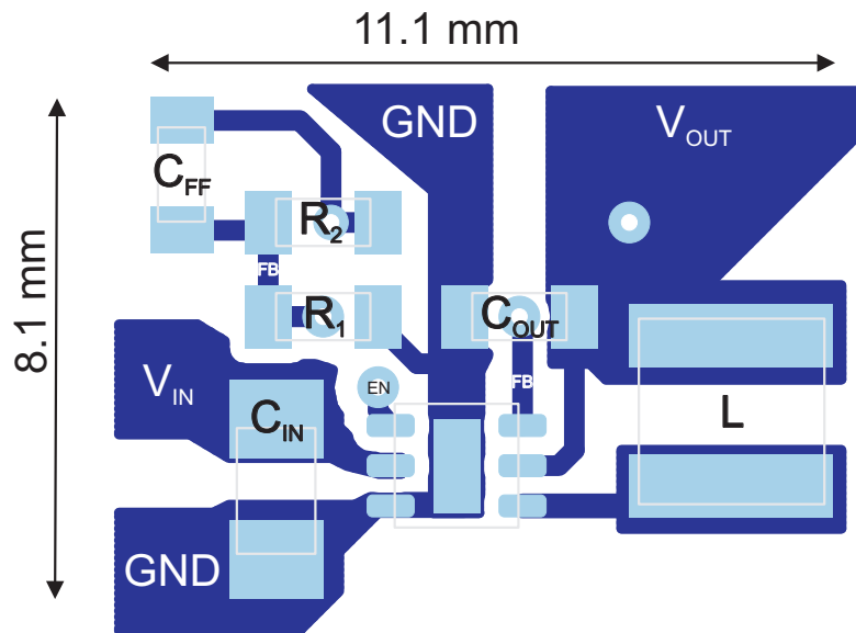
Figure 40. PCB Layout - DRV Package
