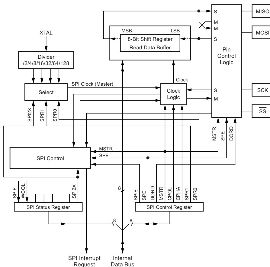
Figure 19-1. SPI Block Diagram (1)
