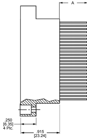
Receptacle Assembly
