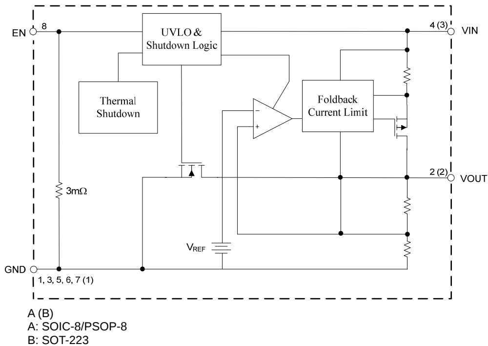
Figure 3. Functional Block Diagram of AP2111 for Fixed Version
