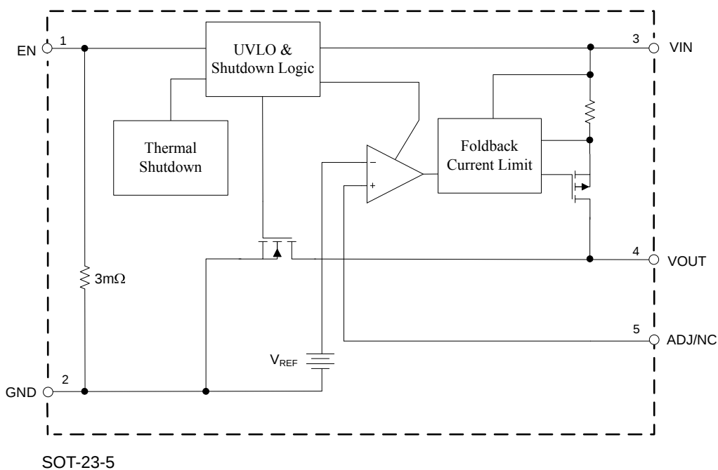
Figure 4. Functional Block Diagram of AP2111 for Adjustable Version
