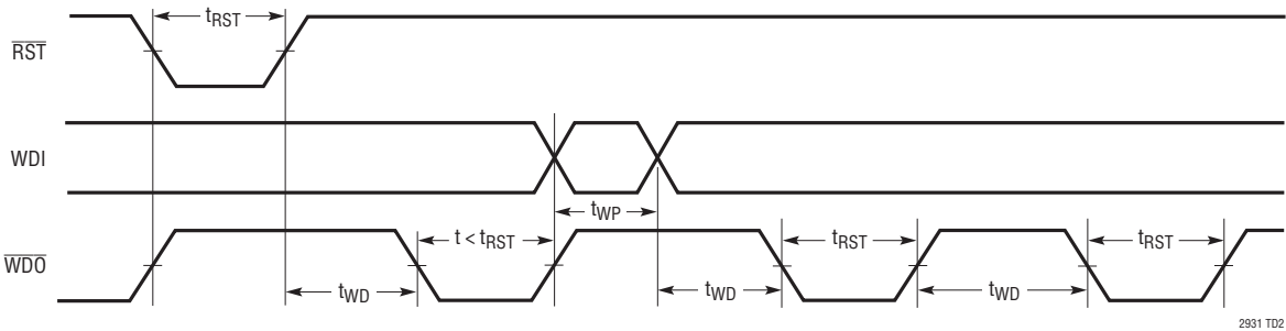
Watchdog Timing
