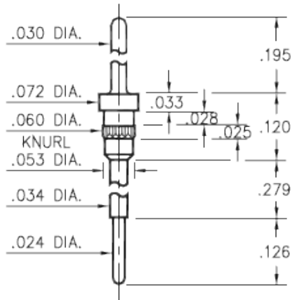
5107-0-00-XX-00-00-03-0 Press-fit in .057 mounting hole
