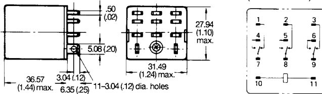
Terminal arrangement (Bottom view)
