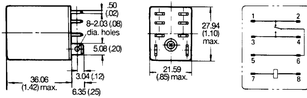
Terminal arrangement (Bottom view)
