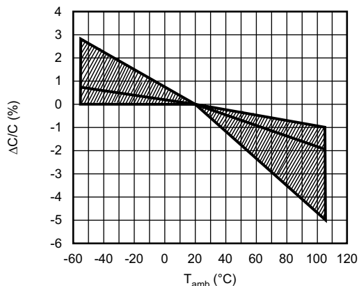
Capacitance as a function of ambient temperature (typical)
