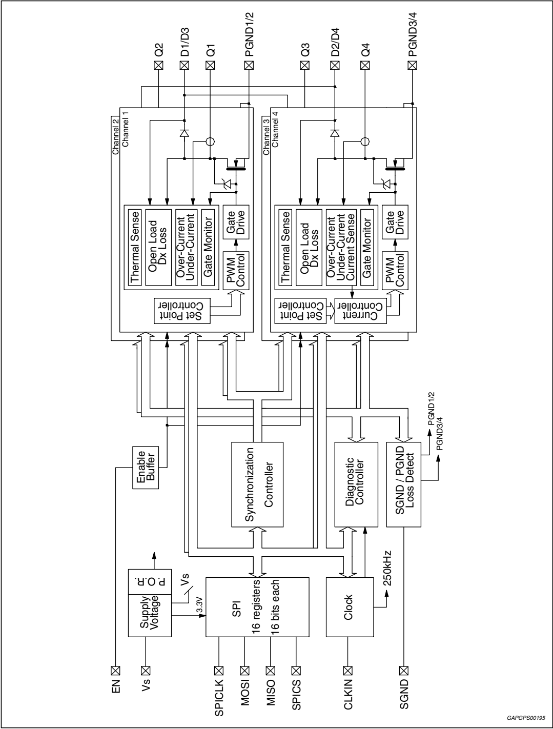
Figure 1. Block diagram
