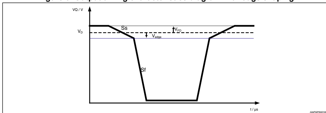
Figure 5. Output timing characteristics diagram with edge shaping
