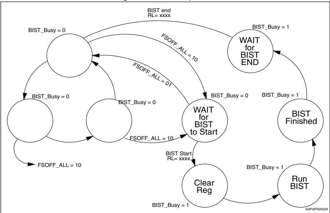
Figure 30. BIST sequence
