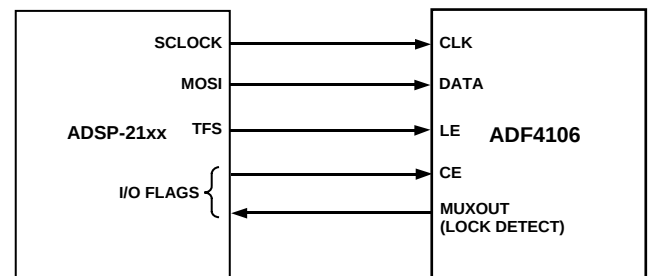
Figure 24. ADSP-21xx-to-ADF4106 Interface
