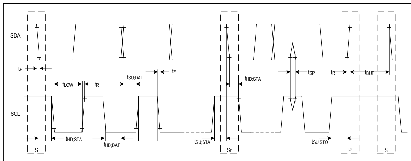
Figure 72. 2-Wire Bus Timing Diagram
