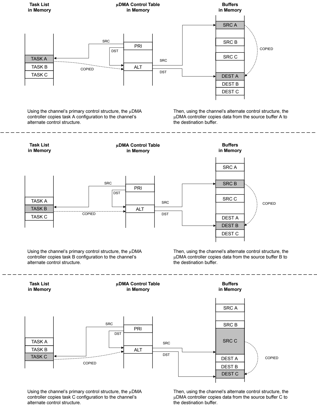
Figure 7-4. Memory Scatter-Gather, μDMA Copy Sequence
