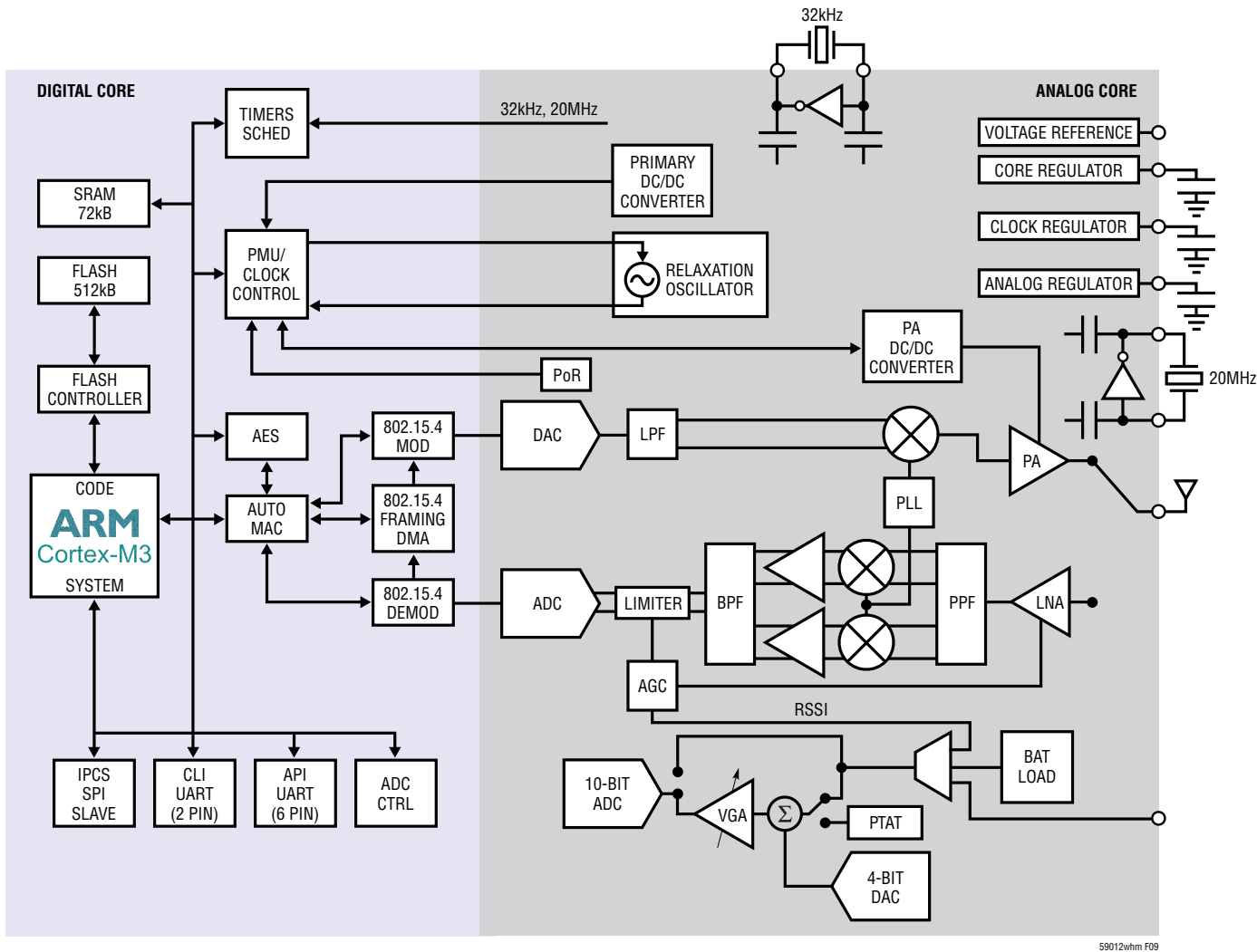
Figure 9. Eterna Block Diagram
