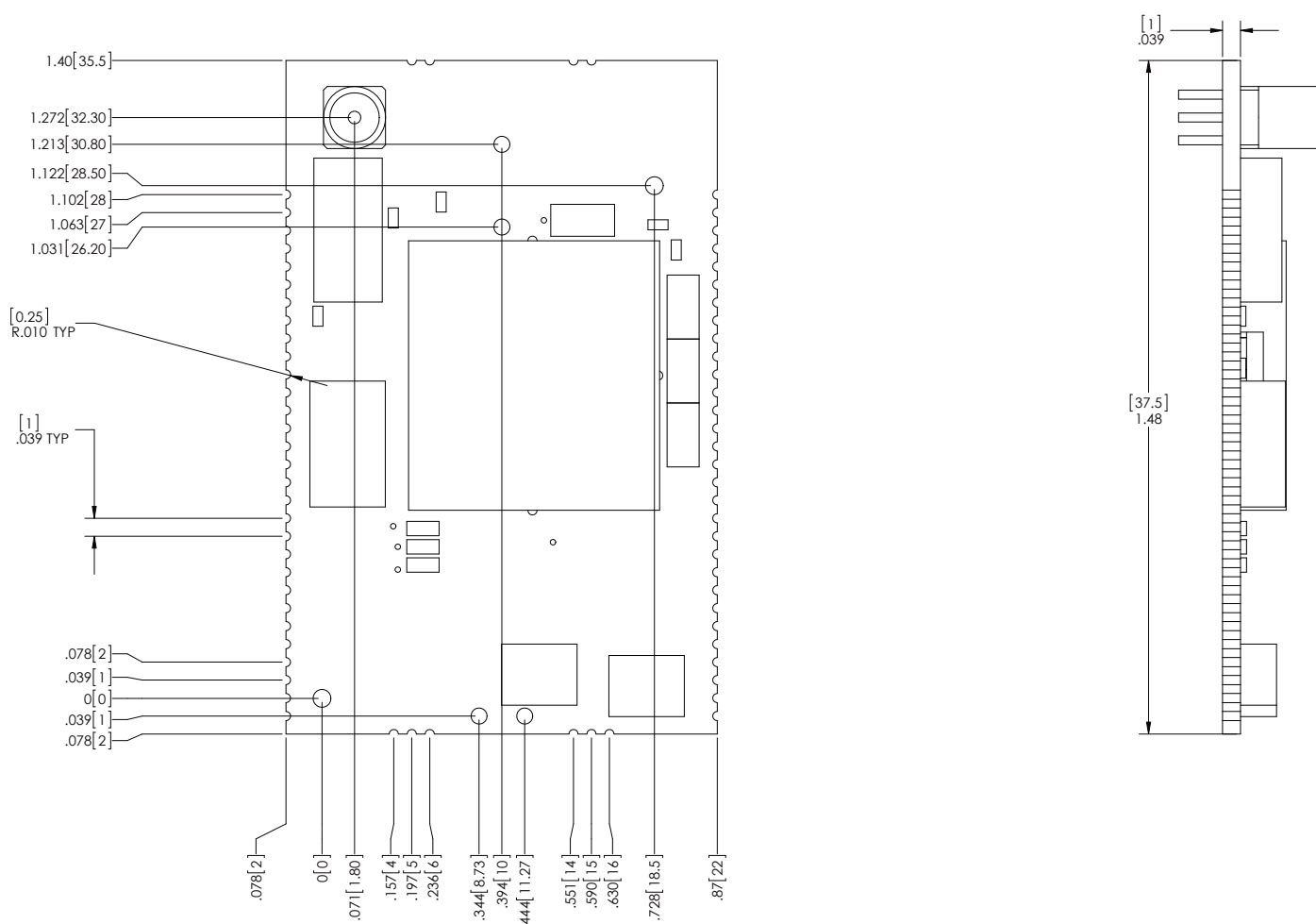
Figure 13. LTP5902 Mechanical Drawing
