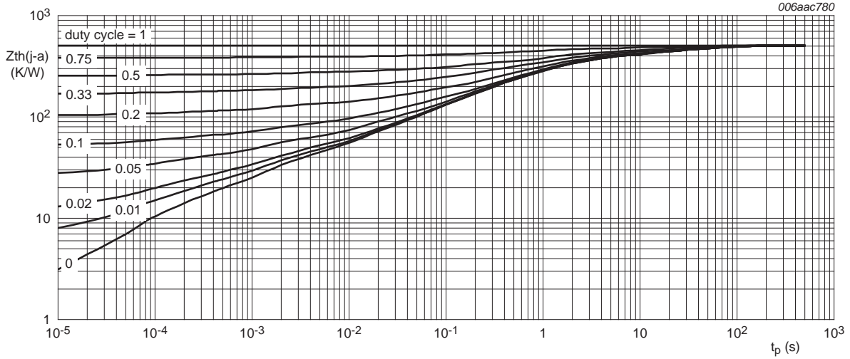
Fig 5. Transient thermal impedance from junction to ambient as a function of pulse duration for PDTA124EU (SOT323); typical values
