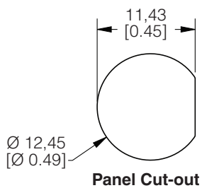
Figure 2. Panel Cutout
