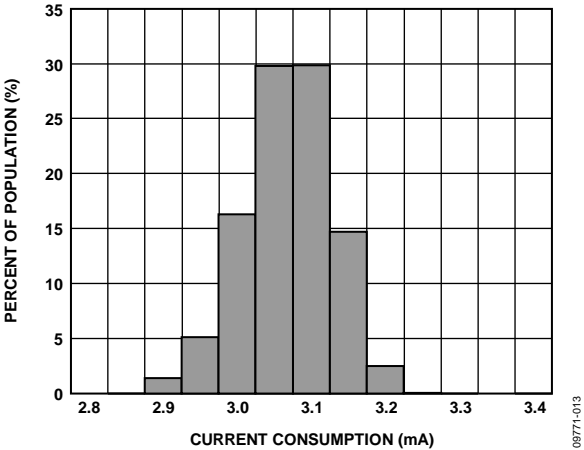
Figure 18. Current Consumption at 25°C ( V_{RATIO} = 5\text{ V} )
