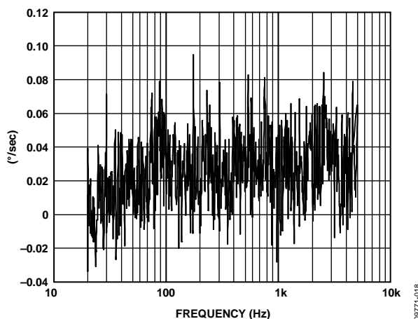
Figure 22. ADXRS646 Sine Vibration Output Response (5 g, 20 Hz to 5 kHz); Gyroscope Bandwidth Set to 1600 Hz
