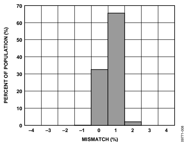
Figure 12. Self-Test Mismatch at 25°C ( V_{\text{RATIO}} = 5 \text{ V} )
