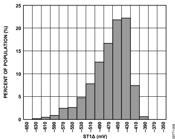
Figure 10. ST1 Output Change at 25°C ( V_{\text{RATIO}} = 5 \text{ V} )
