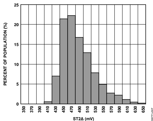
Figure 13. ST2 Output Change at 25°C ( V_{\text{RATIO}} = 5 \text{ V} )
