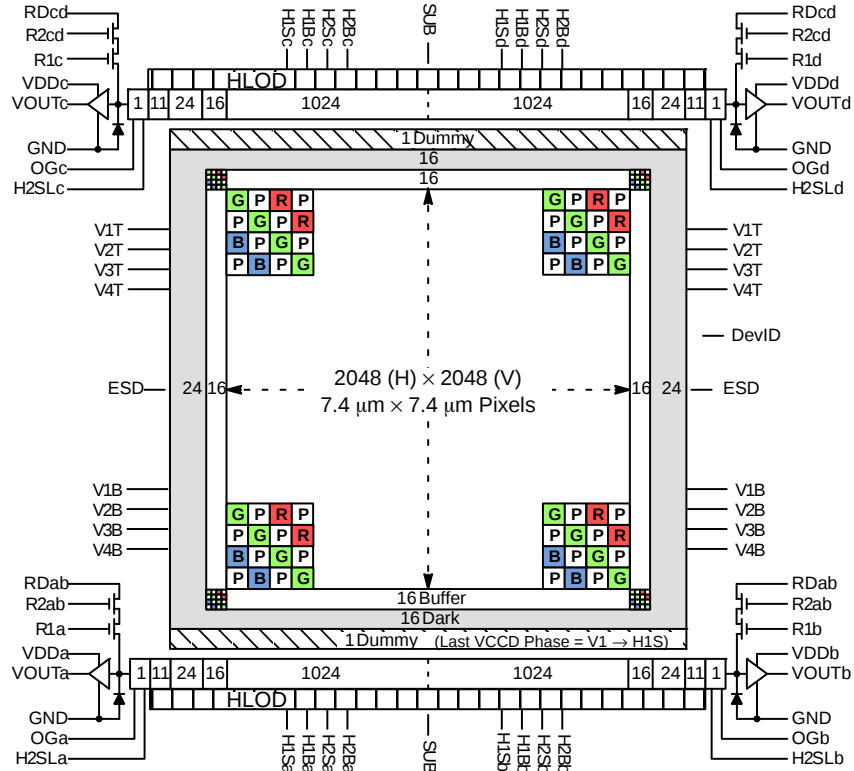
Figure 4. TRUESENSE Sparse Color Filter Pattern
