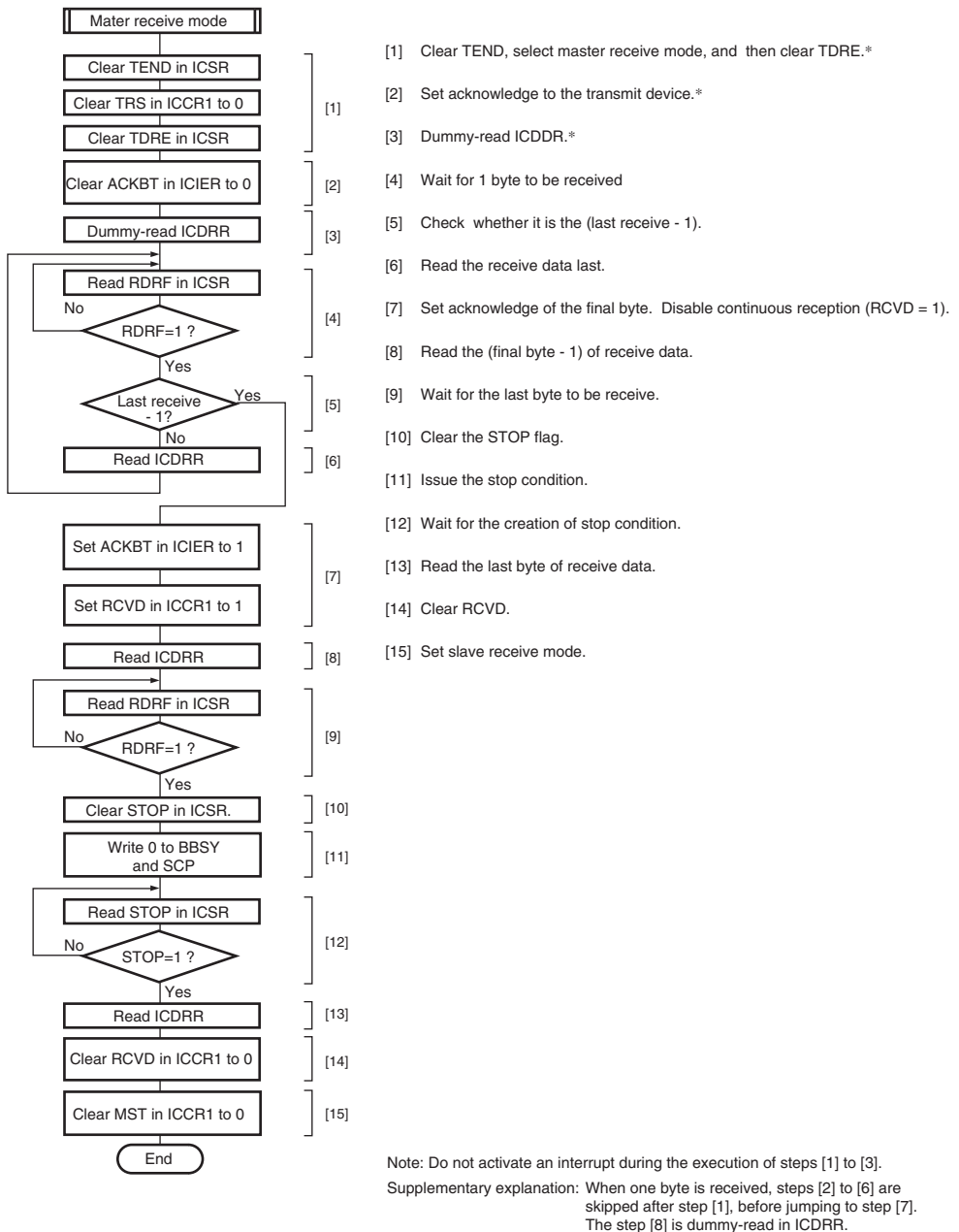
Figure 17.18 Sample Flowchart for Master Receive Mode
