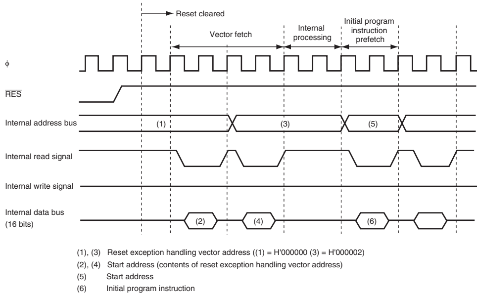
Figure 3.1 Reset Sequence
