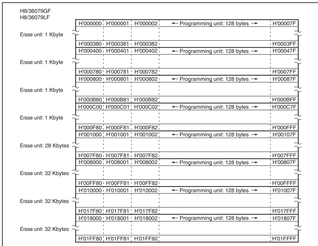
Figure 7.1 Flash Memory Block Configuration (1) (H8/36079GF and H8/36079LF)
