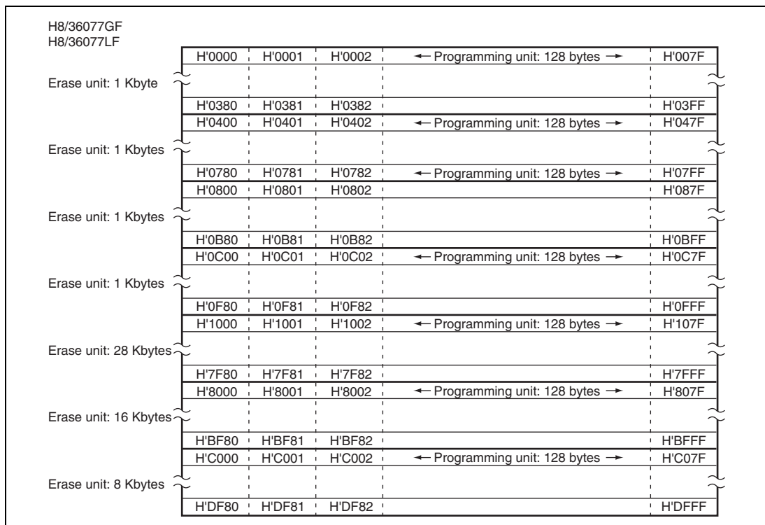
Figure 7.1 Flash Memory Block Configuration (3) (H8/36077GF and H8/36077LF)
