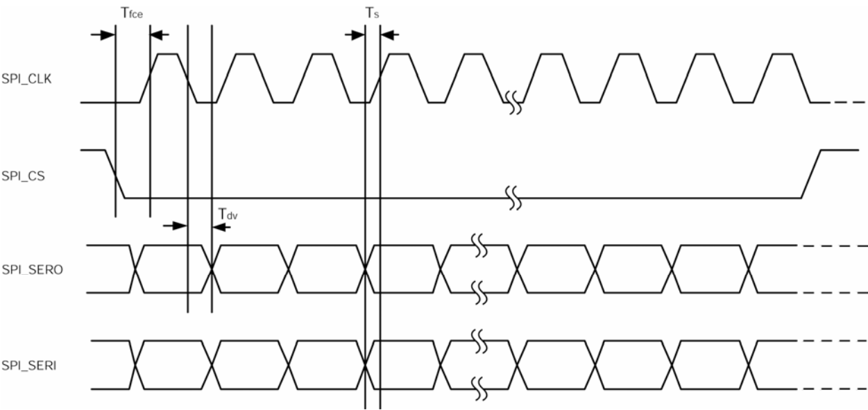
Figure 31: SPI Port Timing Diagram
