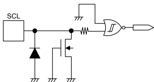
Figure 17 SCL Pin
