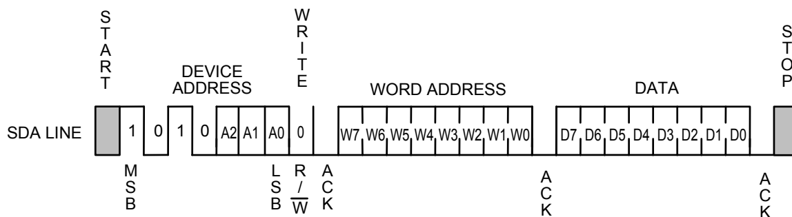
Figure 9 Byte Write
