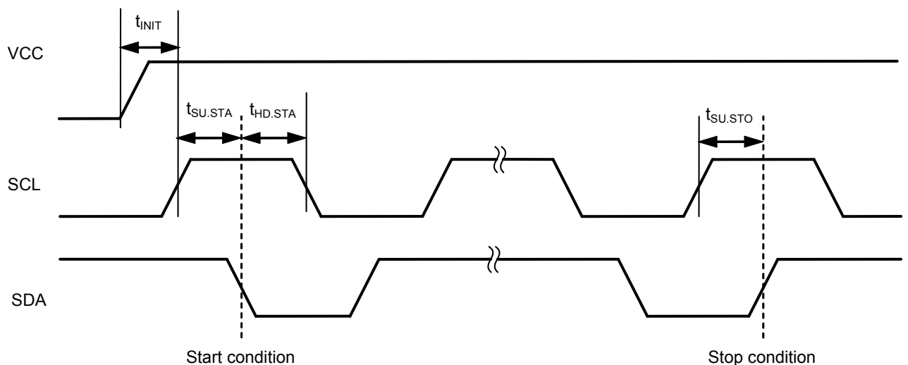
Figure 5 Start / Stop Conditions after Power-on
