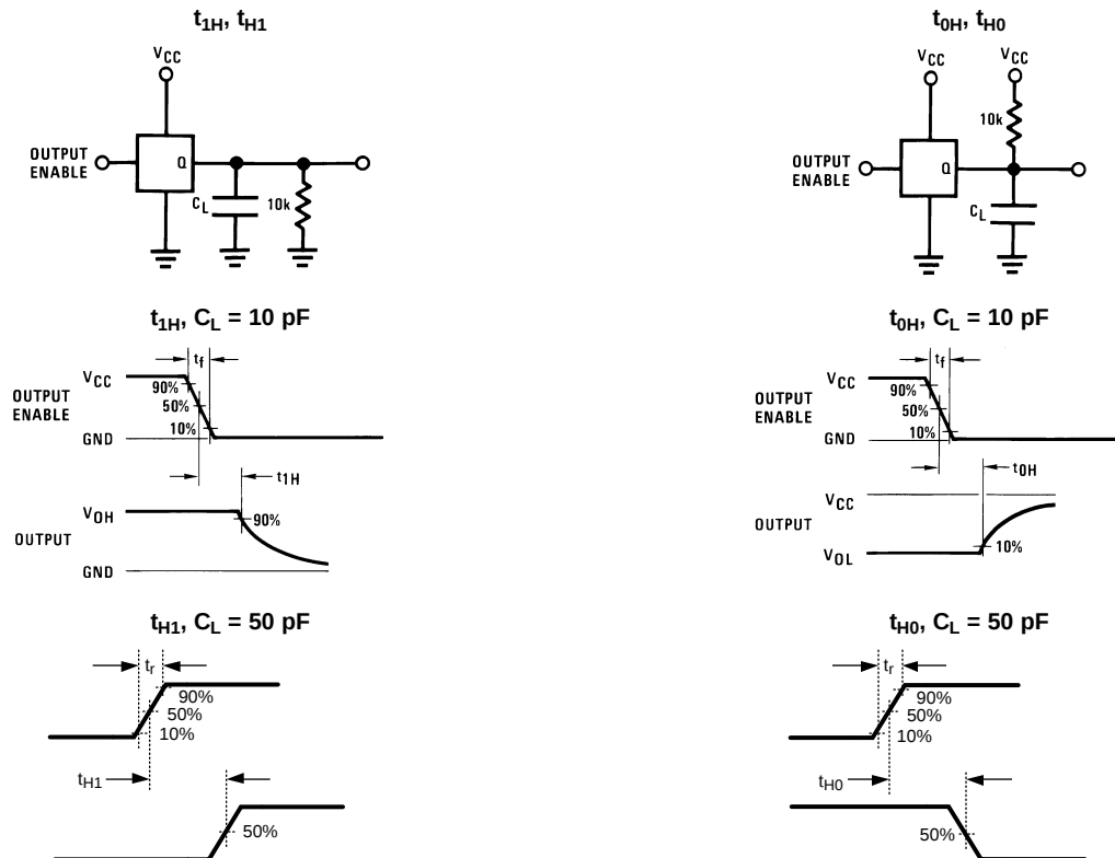
Figure 10. TRI-STATE Test Circuits and Timing Diagrams
