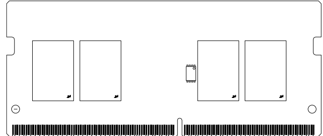
Figure 1: 260-Pin SODIMM (MO-310 R/C A1, R/C A2)
