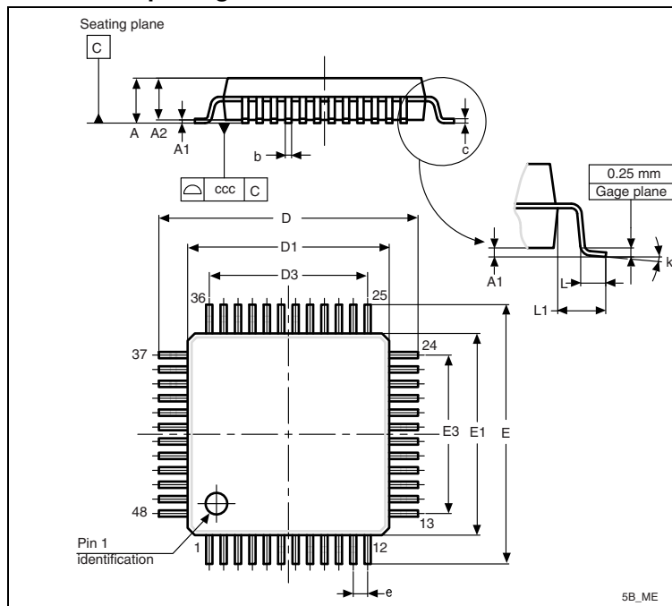
Figure 32. LQFP48 – 7 x 7 mm, 48-pin low-profile quad flat package outline (1)
