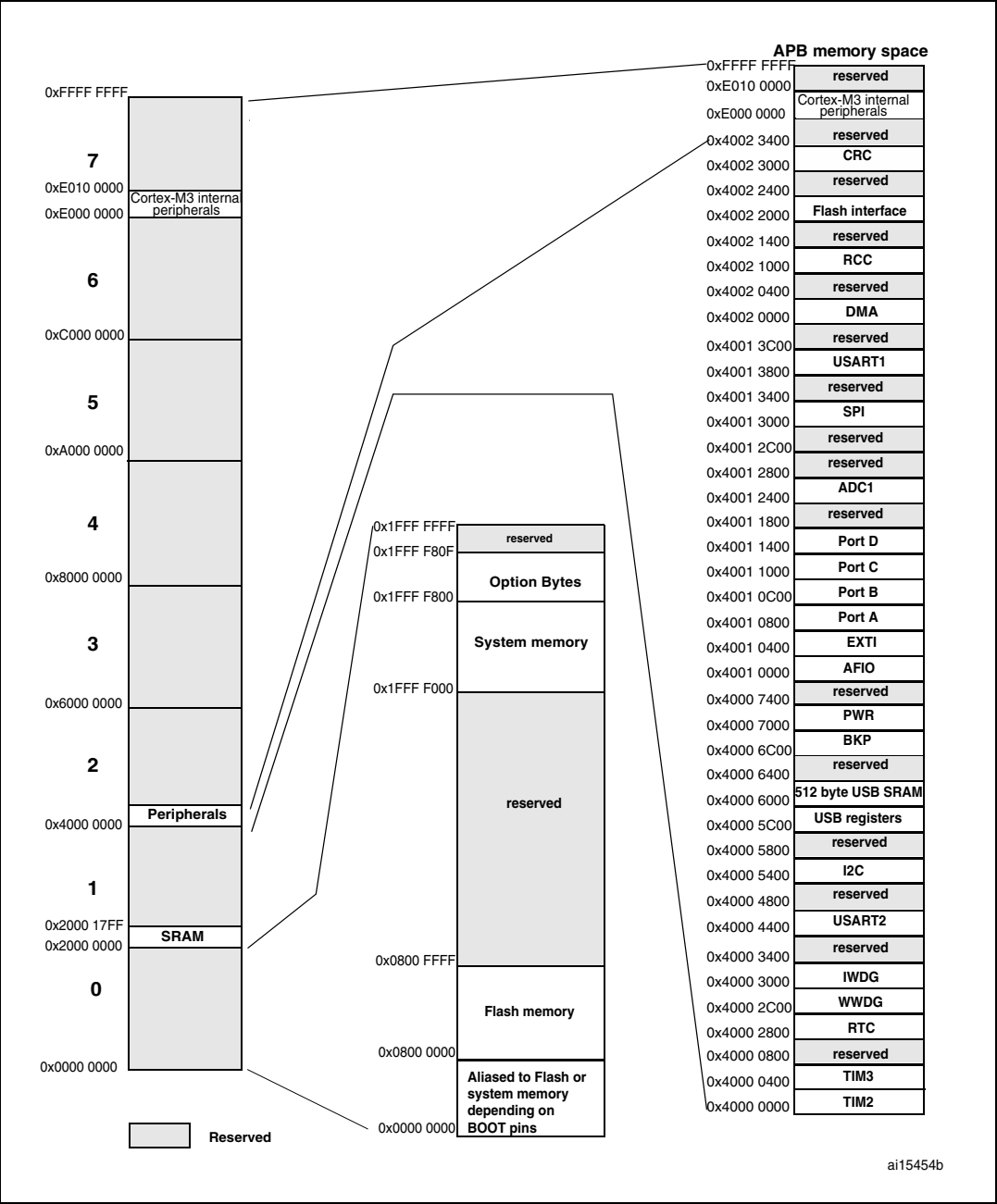
Figure 5. Memory map
