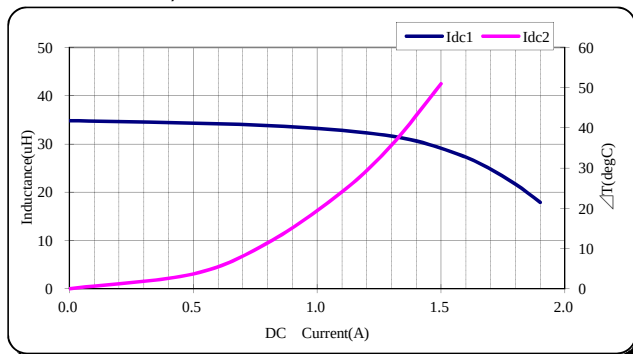
TDK' PartNo.;VLS5045EX-330M
