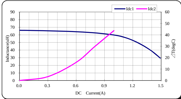
TDK' PartNo.;VLS5045EX-680M
