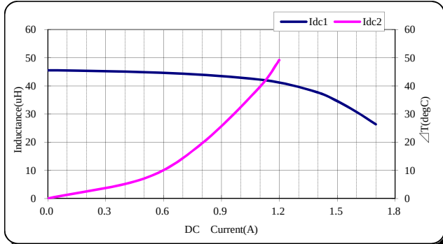
TDK' PartNo.;VLS5045EX-470M
