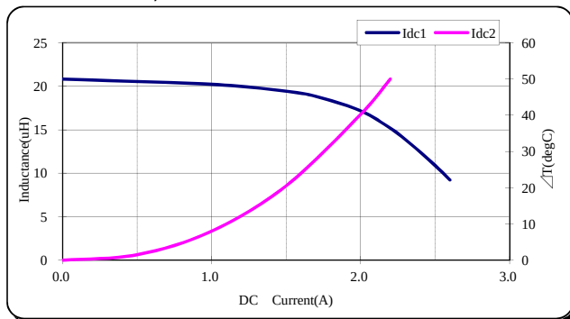
TDK' PartNo.;VLS5045EX-220M
