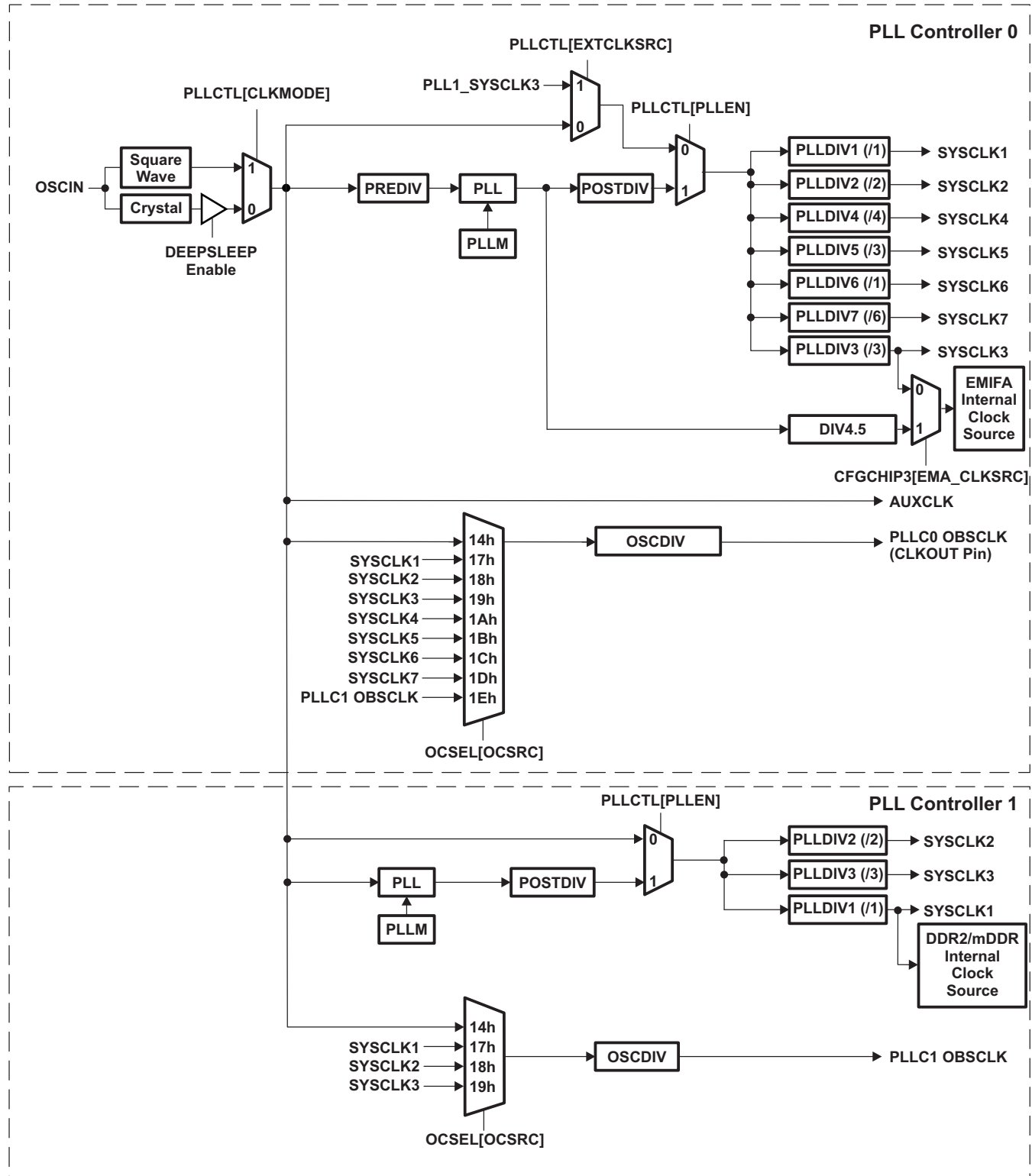
Figure 6-9. PLL Topology
