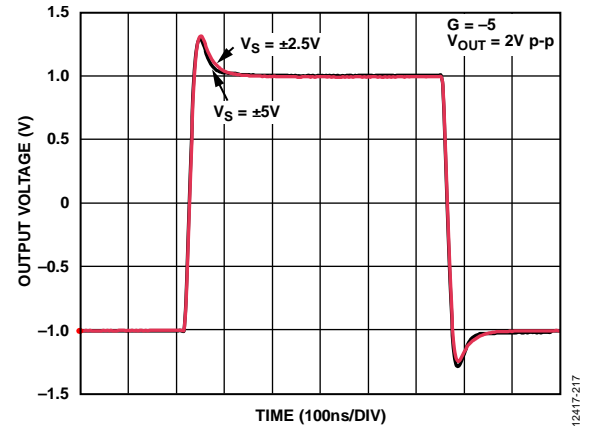
Figure 19. Large Signal Step Response for Various Supplies, G = -5
