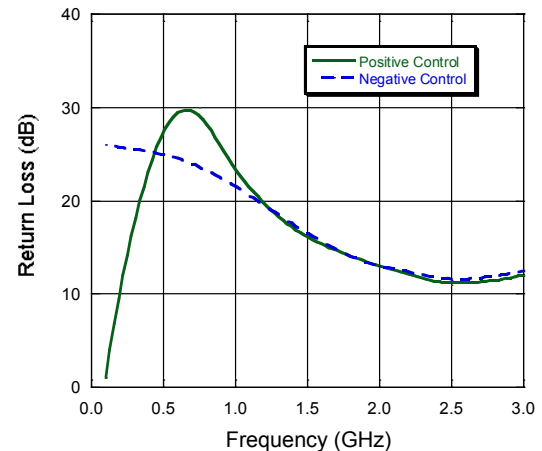
Return Loss (10 dB State)
