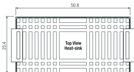
Dimension Drawing with Heat-sink (mm)
