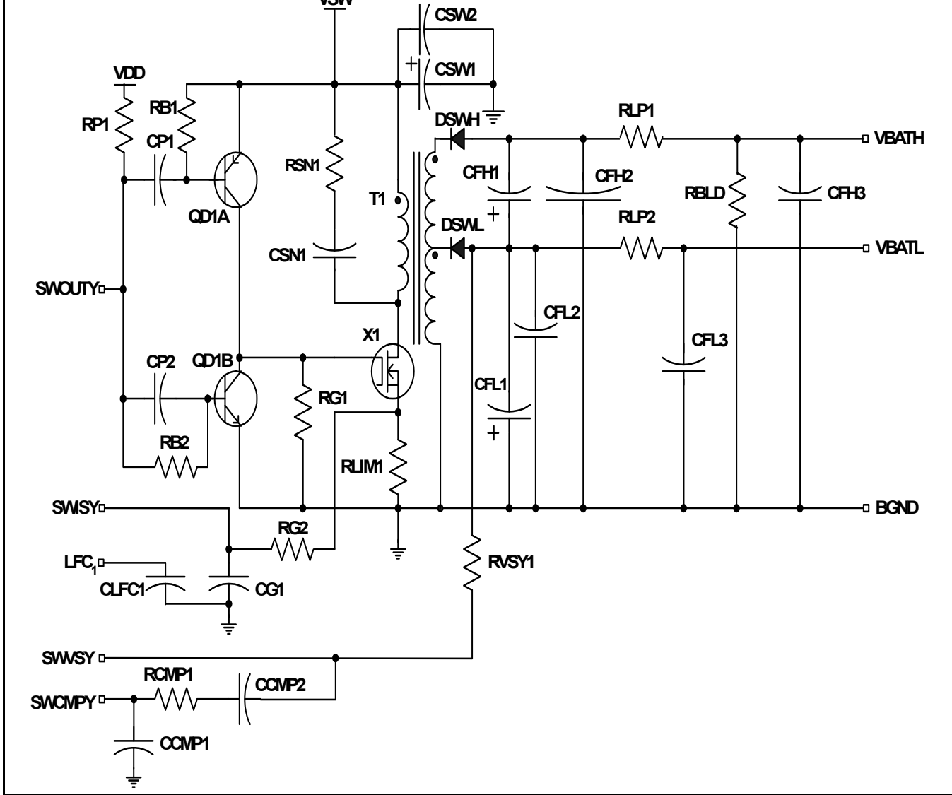
Figure 44 - Le88266/286 Switching Regulator Circuit
