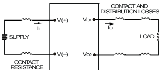
Figure 14. Output Ripple and Noise Test Setup.
