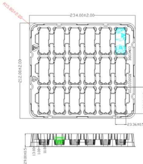
Open Frame Through Hole Pin Module Tray Figure 27. EBDW020 Packaging Tray
