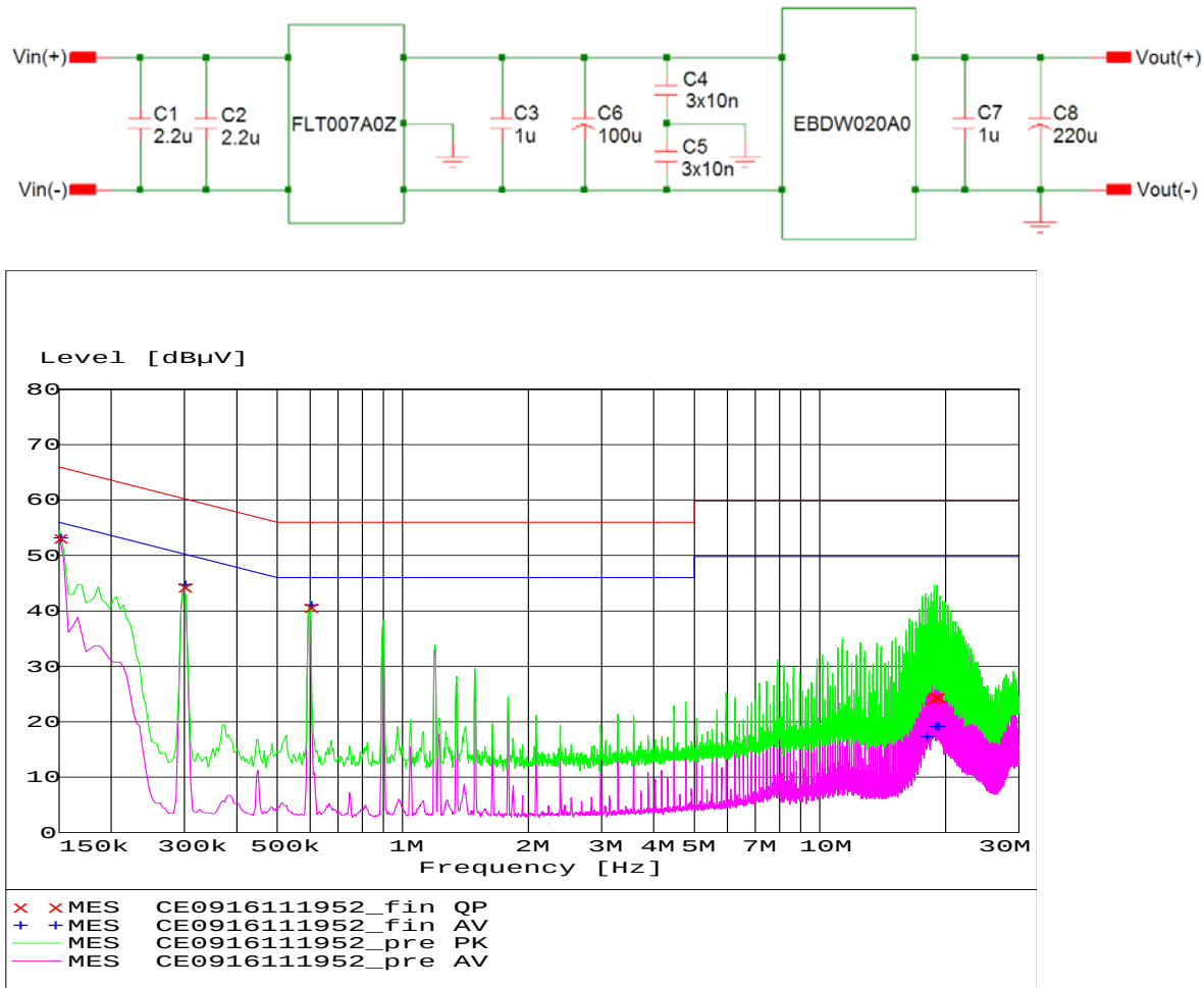
Figure 26. EMC Considerations.
