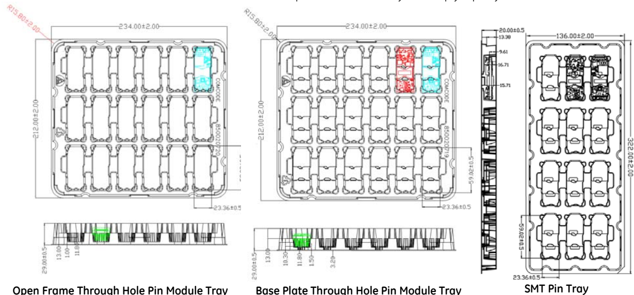
Figure 27. EBDW020 Packaging Tray
