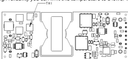
Figure 19. Location of the thermal reference temperature TH 1 . Do not exceed 113 °C.
