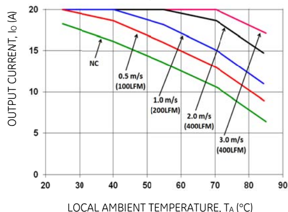
Figure 22. Output Current Derating for the Base Plate EBDW020A0Bxx-H in the Transverse Orientation; Airflow Direction from Vin(-) to Vin(+); Vin = 48V.
