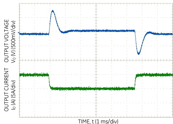
Figure 6. Typical Transient Response to Step Change in Load from 50% to 75% to 50% of Full Load at 48Vdc Input and C_o = 470uF Polymer, without -02 option.
