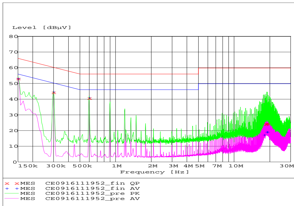
Figure 26. EMC Considerations.
