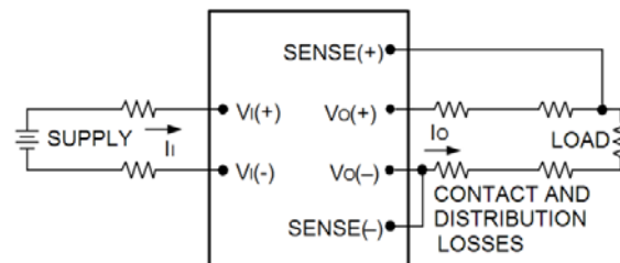
Figure 17. Circuit Configuration for remote sense.
