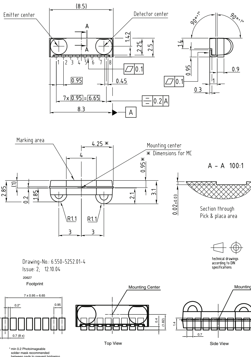
Fig. 8 - Package Drawing
