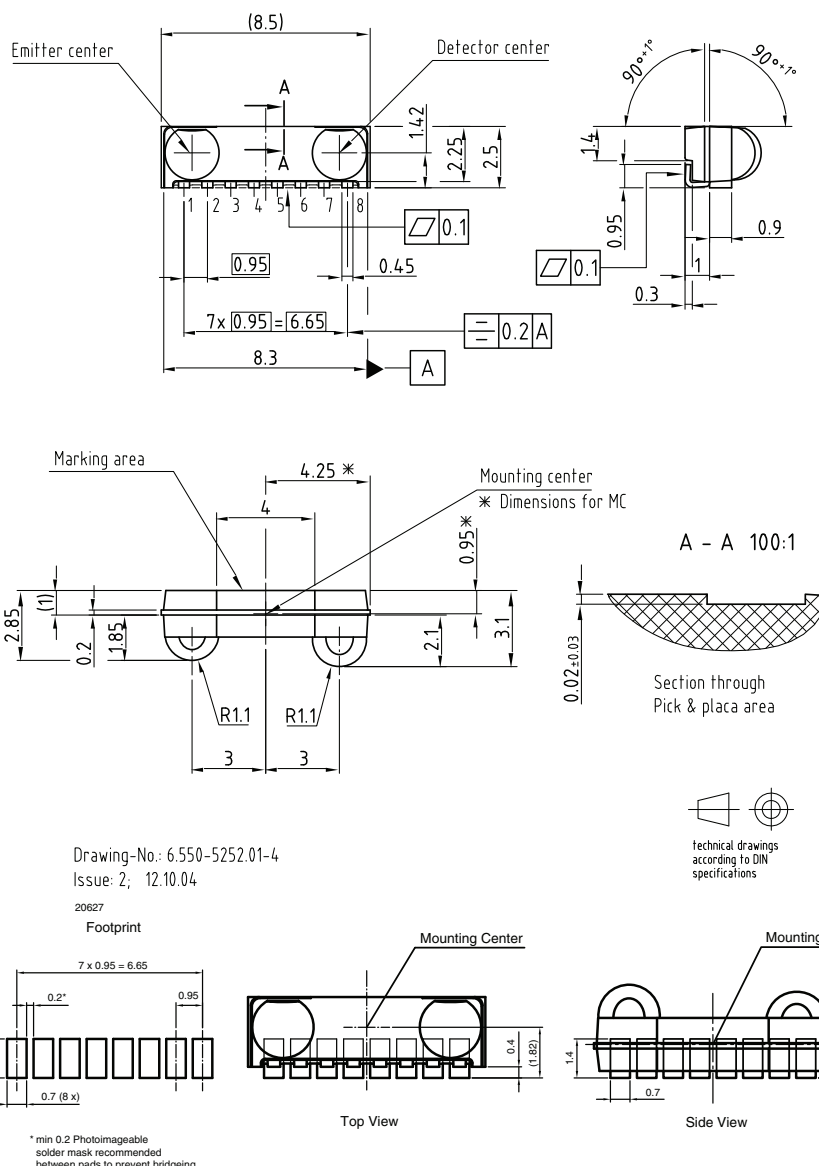
Fig. 8 - Package Drawing
