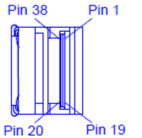
View "Y"
