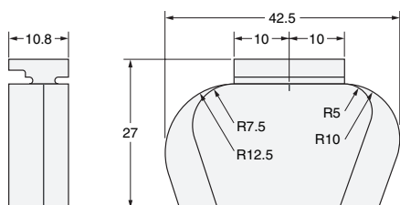
Mounting Bracket E39-L83
