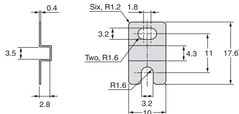
Mounting Bracket E39-L83
