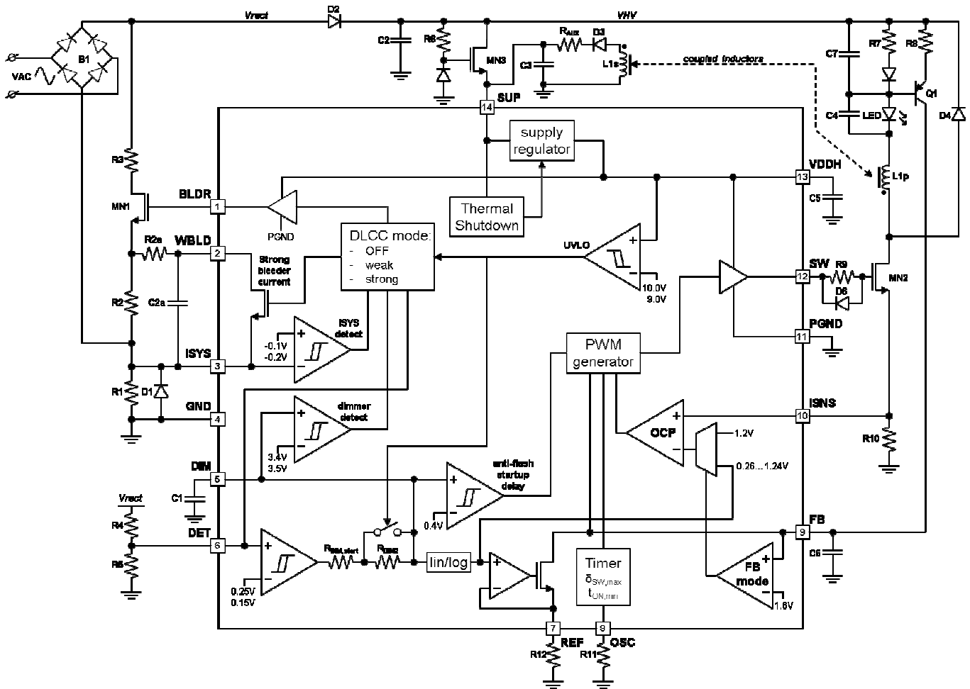
Figure 4. Block diagram of BD555BKFV functions
