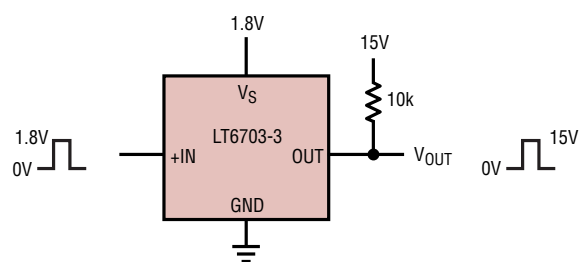
Level Translator Low Voltage to High Voltage
