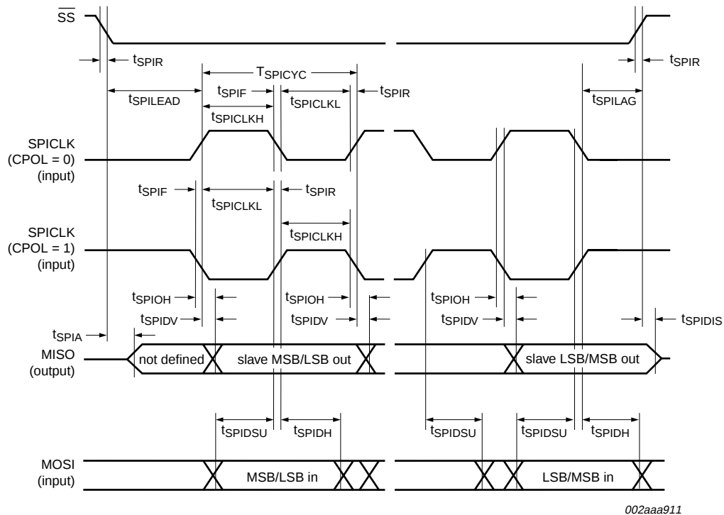
Fig 30. SPI slave timing (CPHA = 1)
