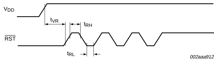
Fig 31. ISP entry timing
