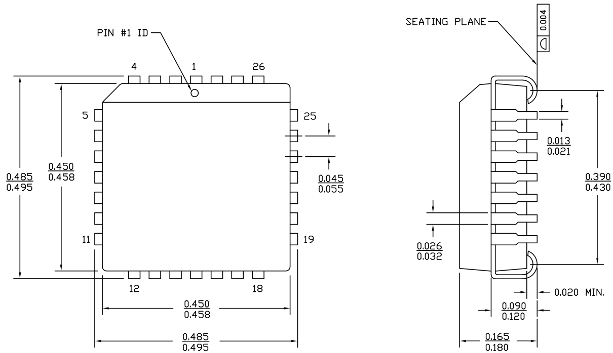
Figure 13. 28-Pin Plastic Leaded Chip Carrier J64
