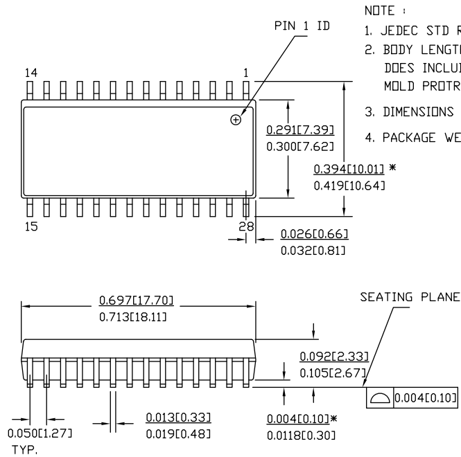
Figure 14. 28-Pin (300-Mil) Molded SOIC S21
