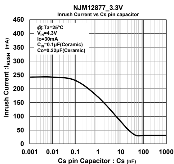
Inrush Current vs. Cs Pin Capacitor
