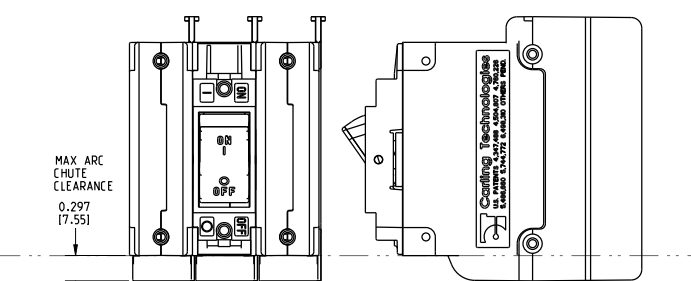
3-POLE (CF3,CG3,C13,C23) w/ ARC CHUTE BARRIER
