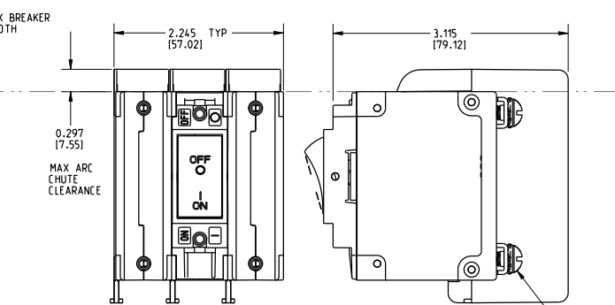
3-POLE (CC3,CD3) w/ ARC CHUTE BARRIER
