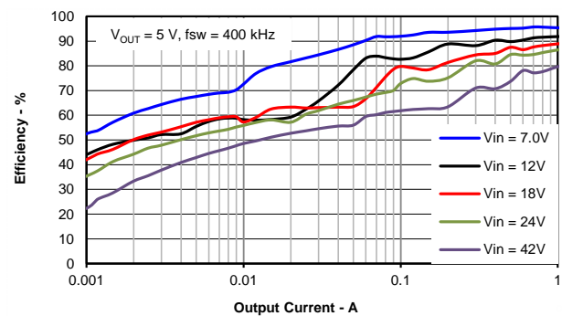
Figure 4. Light-Load Efficiency
