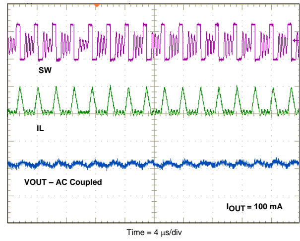
Figure 13. Output Voltage Ripple DCM
