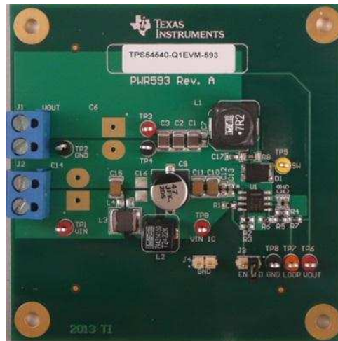
Figure 1. TPS54540-Q1EVM-593 Board
