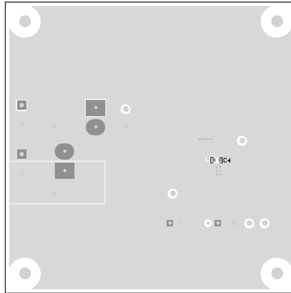
Figure 27. TPS54540-Q1EVM-593 Bottom-Side Assembly and Silkscreen (Viewed From Top)
