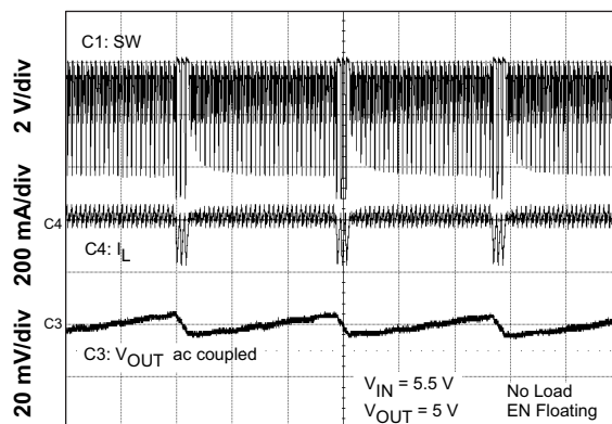
Time = 20 \mu s/div Figure 22. Low Dropout Operation
