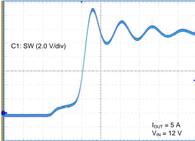
Figure 15. SW Voltage Without Snubber
