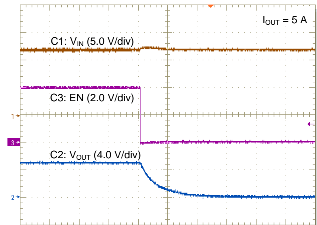
Time: 200 \mu s/div Figure 21. Shutdown Relative to EN
