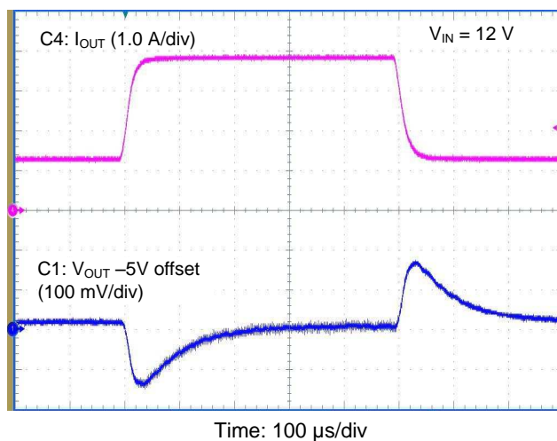
Figure 7. Load Transient Response
