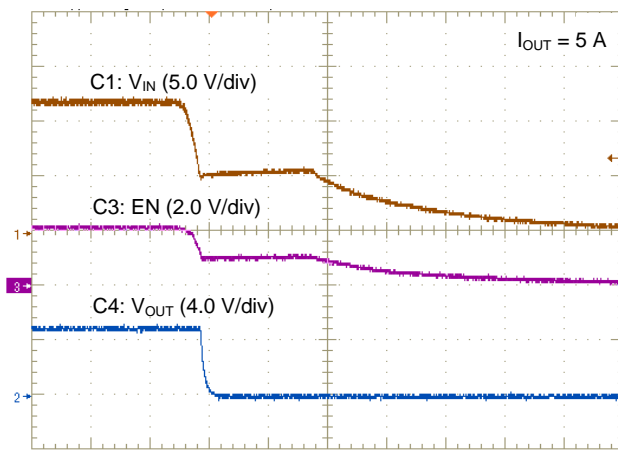
Time: 2.0 ms/div Figure 20. Shutdown Relative to V_{IN}
