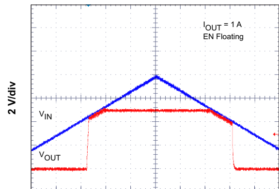
Time = 40 \mu s/div Figure 23. Low Dropout Start Up and Shutdown
