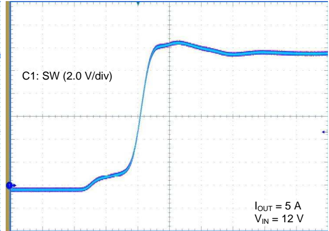
Figure 16. SW Voltage With Snubber
