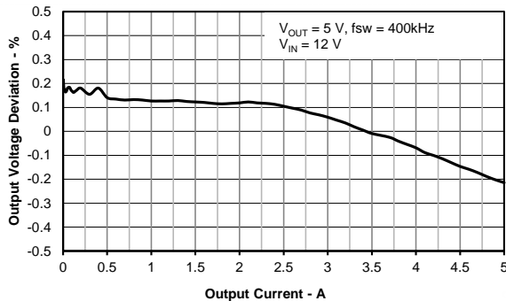
Figure 5. Regulation versus Output Current
