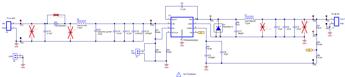
Figure 2. TPS54540-Q1EVM-593 Schematic
