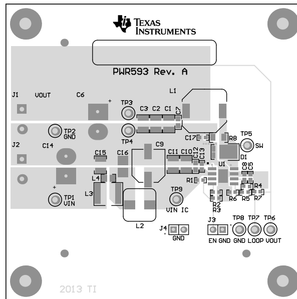
Figure 24. TPS54540-Q1EVM-593 Top Assembly and Silkscreen
