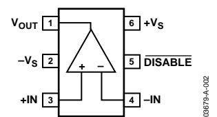
Figure 2. SC70-6 (KS)
