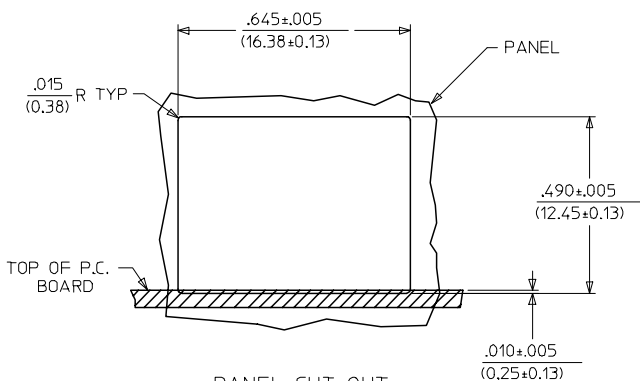
PANEL CUT-OUT (0.2 (SHIELDED W/O BOTTOM GROUND TABS)
